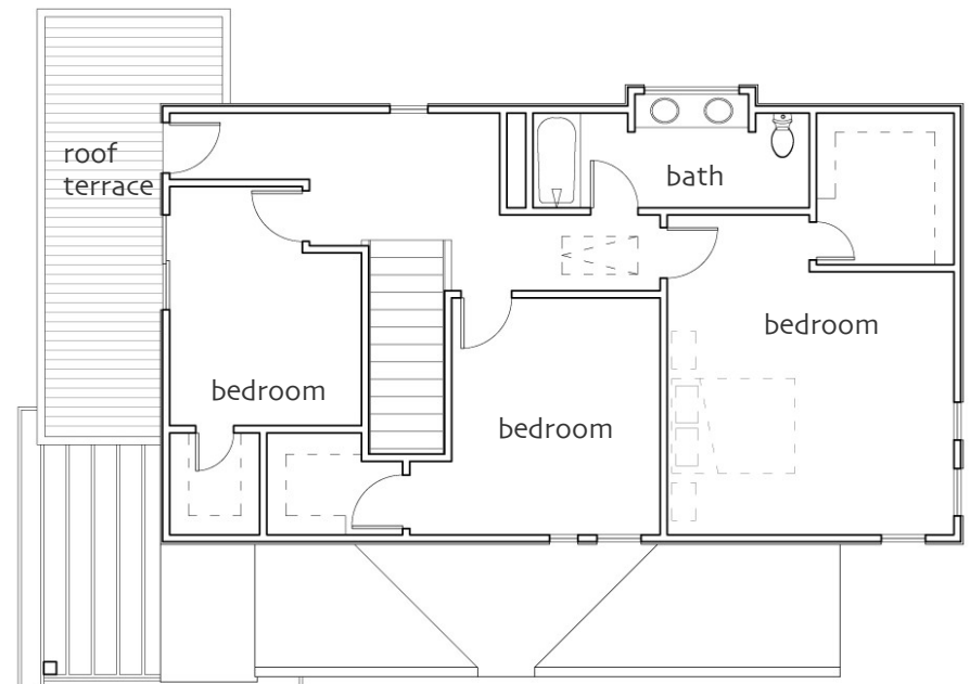
second floor
